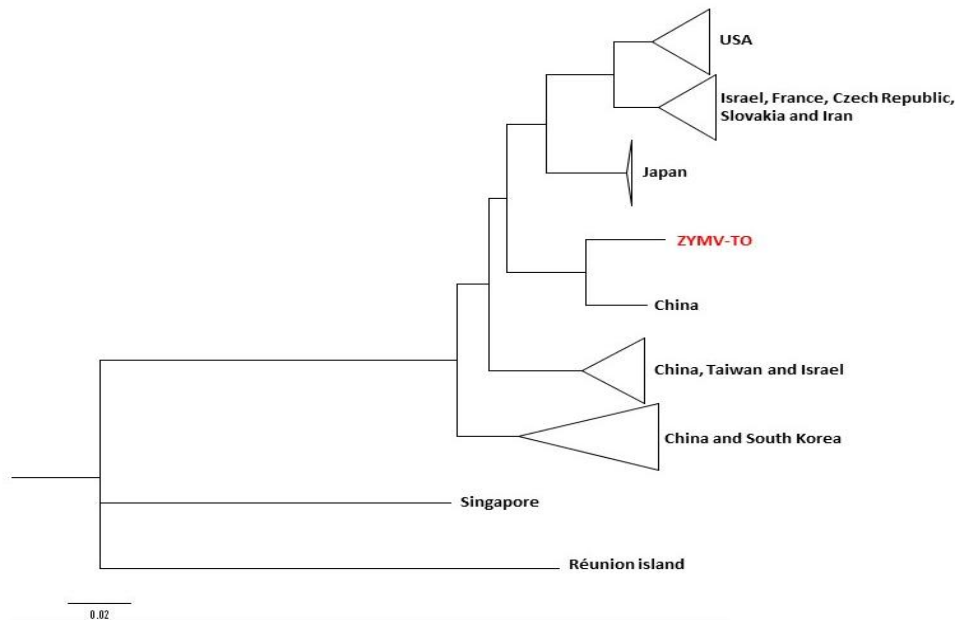
Fig. 2. Phylogenetic analysis of ZYMV-TO. Phylogenetic tree showing ZYMV-TO and 63 complete nucleotide sequences of the ZYMV viral genome. Built by the Maximum Likelihood method, PhyML 3.0 program. The bar at the bottom of the left side shows the number of substitutions/sites. The tree was rooted by midpoint . Some branches were collapsed for better visualization
