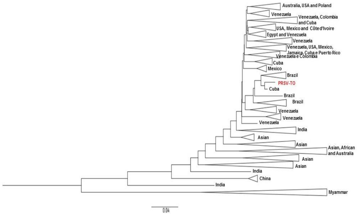
Fig. 1A. Phylogenetic analysis PRSV-TO. Phylogenetic tree showing PRSV-TO and 27 complete nucleotide sequences of the PRSV viral genome. Built by the Maximum Likelihood method, PhyML 3.0 program. The bar at the bottom of the left side shows the number of substitutions/sites. The tree was rooted by midpoint . Some branches were collapsed for better visualization
