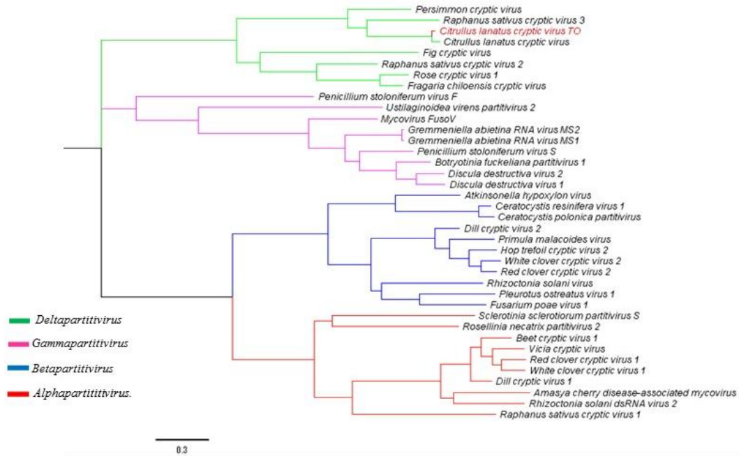
Fig. 4. Phylogenetic analysis of CiLPV-TO (CP) representing RNA1 of the genus Deltapartitivirus . Phylogenetic analysis was performed between CiLPV-TO (red letter) with 37 nts rdrp sequences of members belonging to deltapartitivirus genera; Gammapartitivirus ; Betapartitivirus and Alphapartitivirus . The tree was built by the Maxim likelihood method, PhyML 3.0 program. The bar at the bottom of the left side shows the number of substitutions/sites. The tree was rooted by the midpoint
