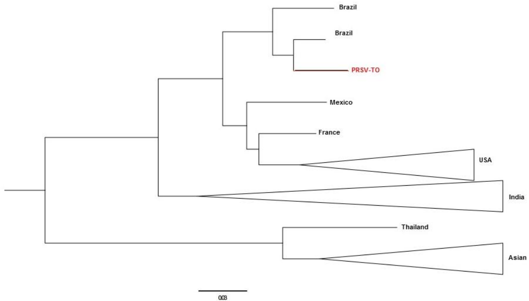
Fig. 1B. Phylogenetic analysis of PRSV-TO (CP). Phylogenetic tree showing PRSV-TO (CP) and 631 nucleotide cp sequences (PRSV). Built by the Maximum Likelihood method, PhyML 3.0 program. The bar at the bottom of the left side shows the number of substitutions/sites. The tree was rooted by the midpoint . Some branches were collapsed for better visualization
