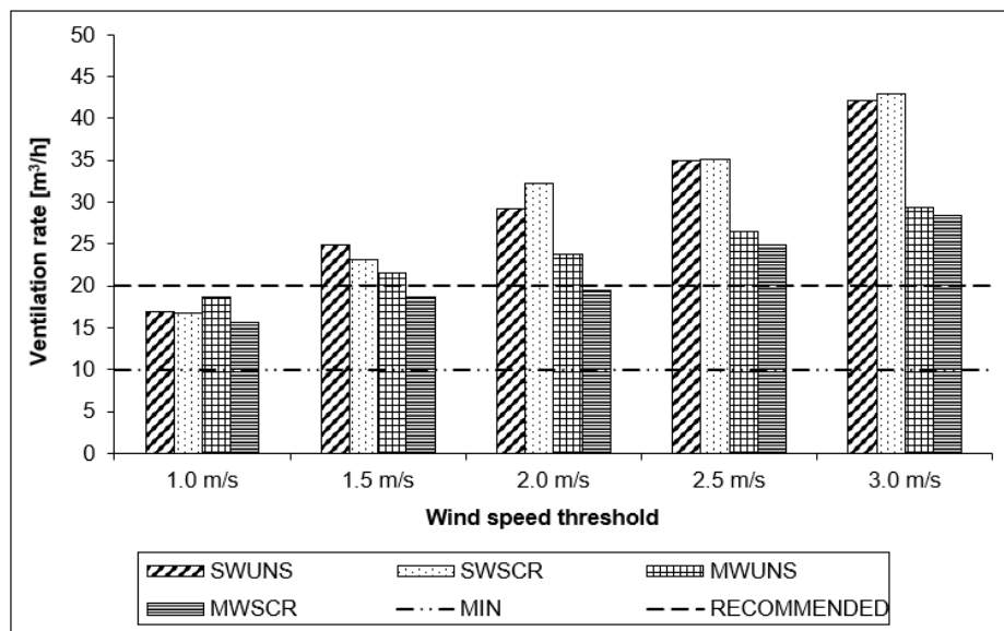
Fig. 2. Ventilation rates ( m^3/h ) in a 100 mm PVC vent pipe fitted to different designs of VIP latrines at varying wind speed thresholds
