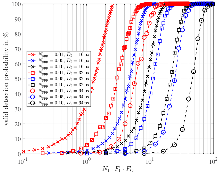
Figure 1. Valid vector detection probability as a function of the effective number of particle images N_1 F_1 F_O for synthetic PIV images with zero in-plane motion ( F_1 = 1 ) and varying out-of-plane motion ( F_O = 0 \dots 1 ) for different particle image densities N_{ppp} and interrogation window sizes D_1 .
