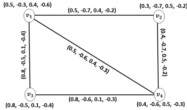
Fig. 2. Bipolar Intuitionistic Anti Fuzzy Graph
