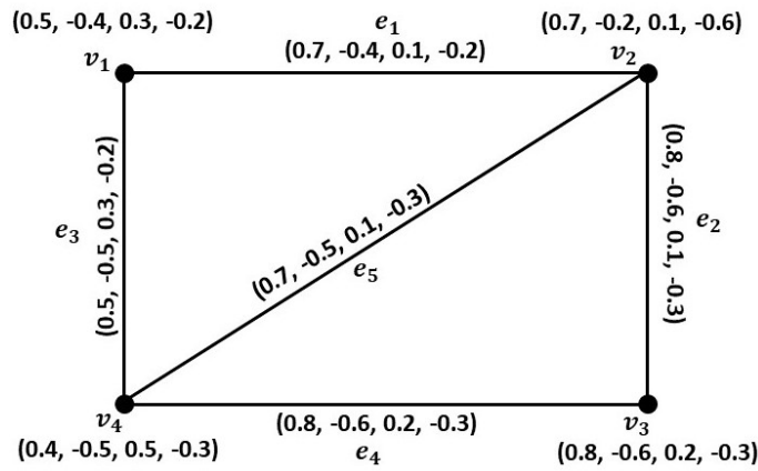
Fig. 3. Edge domination in BIAFG
