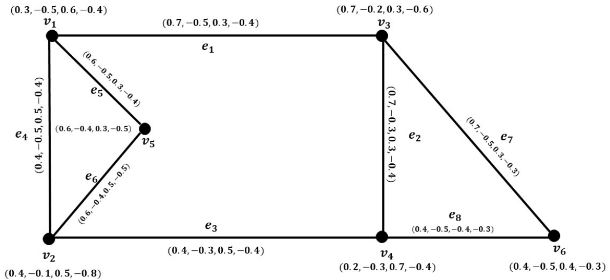
Fig. 4. Secure Edge Domination in BIAFG
