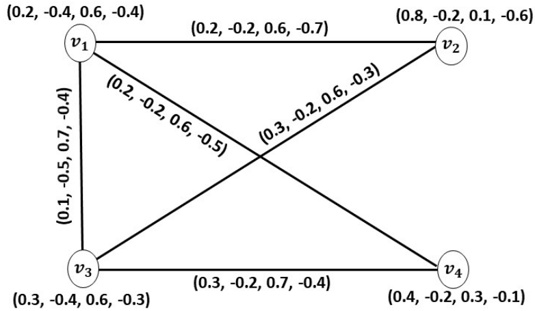
Fig. 1. Bipolar Intuitionistic Fuzzy Graph
