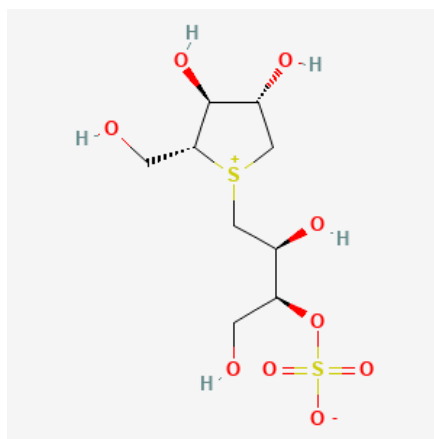
Structure of Kotalanol [37]
