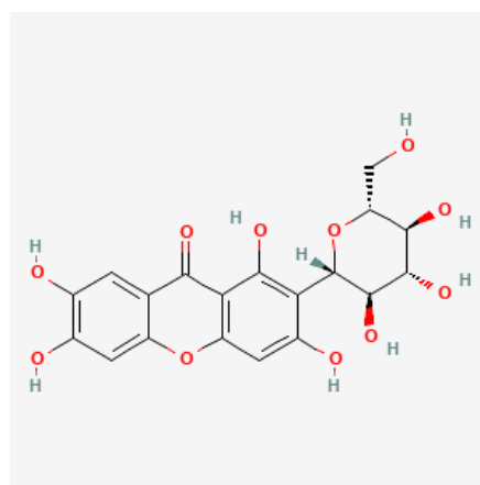
Structure of Mangiferin [36]
