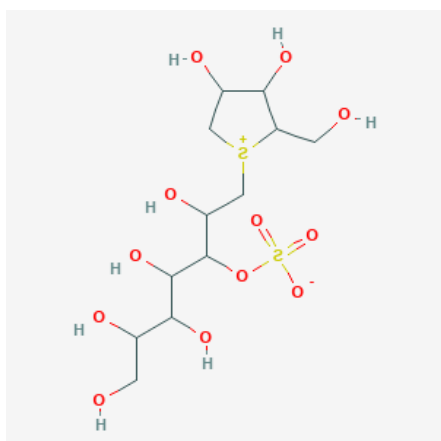
Structure of Salacinol [35]
