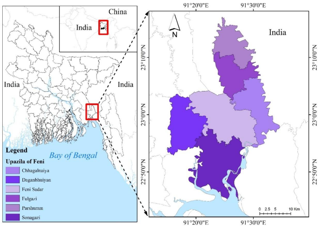
Fig. 1. Sampling points in Feni District, Bangladesh
