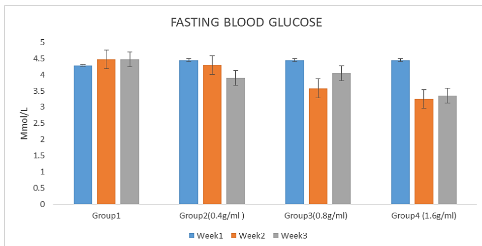
Fig. 1. Variations in the pattern of fasting glucose in the control and caffeine-induced groups
