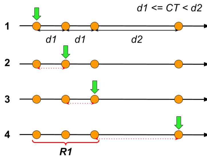
Figure 9. Ranges generation algorithm applied to an example.
