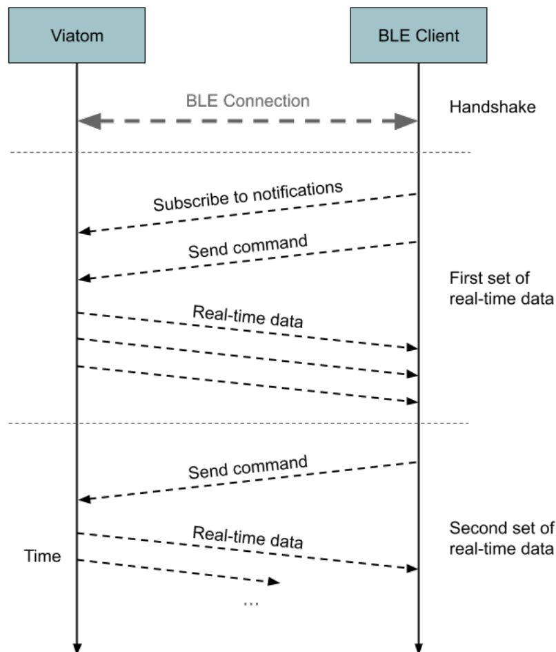
Figure 7. Sequence diagram illustrating the interactions between the Viatom Checkme O2 device and a connected BLE client during the retrieval of real-time data.
