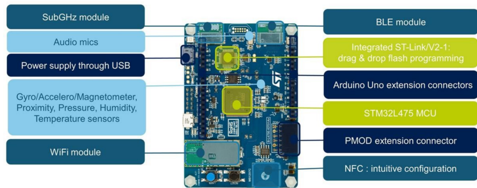
Figure 3. The HDC device block design.
