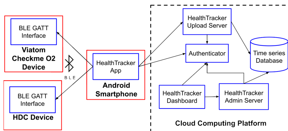
Figure 1. The architecture of HealthTracker.
