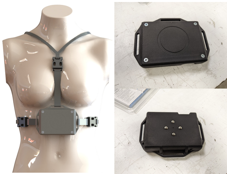
Figure 2. The HDC device. On the left how it is worn, while on the right , we show the front of the device (figure on the top right ) and the back of the device (figure on the bottom right ).
