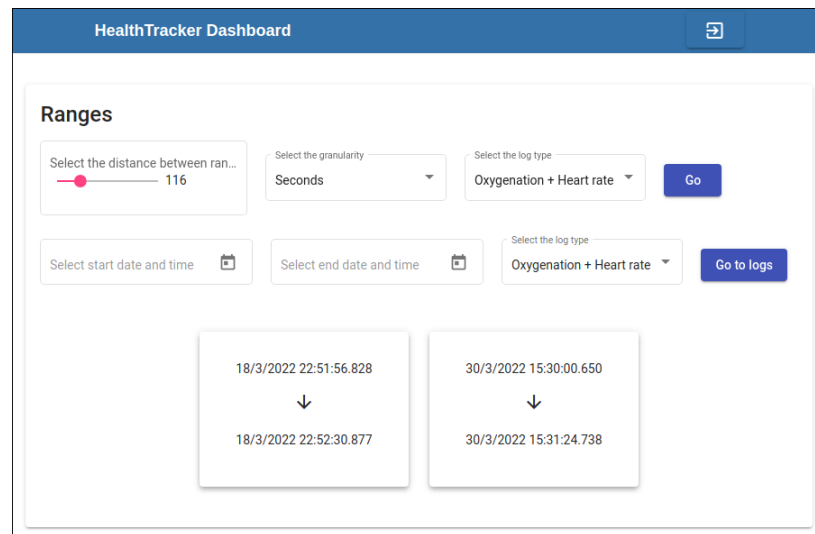
Figure 10. The HealthTracker dashboard page where the logs produced by a specific user can be summarized in configurable time intervals.
