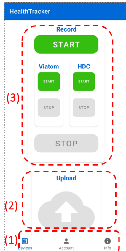
Figure 8. The HealthTracker Android application user interface.
