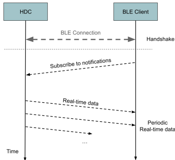
Figure 4. Sequence diagram illustrating the interactions between the HDC device and a BLE client during the retrieval of real-time data.
