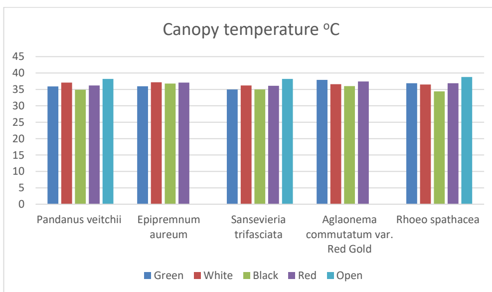
Chart 1. Response of shade net colors, ornamental plants and their interaction on canopy temperature (°C) at 180 DAP during second year
