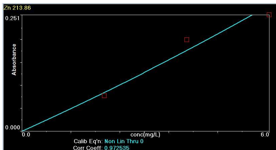
Fig. 1. Calibration curve of zinc with different standards
