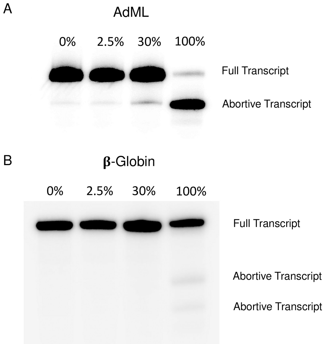
Fig 3. In vitro transcription of AdML and β-Globin. Autoradiograph depicting the T7 polymerase transcription profiles of (A) AdML and (B) β-Globin. Four transcripts of each minigene were created with varying amounts, 0%, 2.5%, 30%, and 100%, of 4sU incorporated. The full pre-mRNA strands and abortive transcripts in each lane are labeled.
